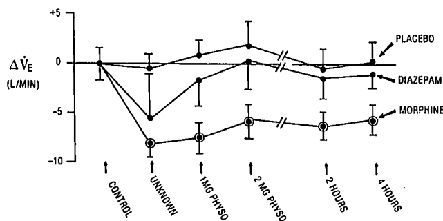
FIG. 1. Isohypercapnic minute ventilation. Values are mean ± 1 SEM. Values at 2 and 4 h were interpolated from \text{CO}_2 -response curves at P_{E\text{T}} = 46 mmHg. Control \dot{V}_E = 14.2 \pm 1.3 l/min. Circled points are different from control ( P < 0.05 ).
