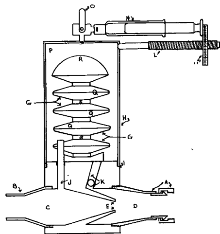
FIG. 1. Side cross section of vaporizer.
