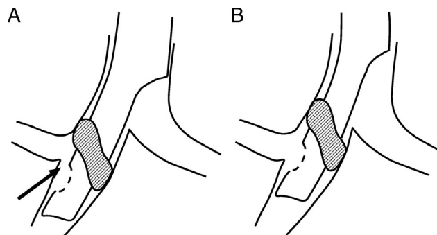
Fig. 1. Scheme for the most distal acceptable position (A) and the most proximal acceptable position (B) of a right-sided double-lumen tube, as defined by Benumof et al. 3 The arrow indicates the space between the wall of the bronchial tip and the bronchial wall.
