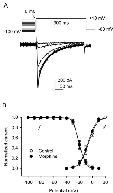
Fig. 3. Absence of effect of morphine ( 0.1 \mu\text{M} ) on voltage-dependent activation and inactivation of L-type \text{Ca}^{2+} current ( I_{CaL} ). (A) Representative current recordings used to determine voltage dependence of I_{CaL} inactivation. Cell was conditioned with 500-ms prepulses from holding potential of -80 \text{ mV} to between -100 and 0 \text{ mV} and back to -80 \text{ mV} for 5 ms, then subjected to 300-ms test pulse to +10 \text{ mV} . (B) Mean values of voltage-dependent activation and inactivation relations for I_{CaL} . No significant differences of V_{0.5} and slope factor were observed for activation and inactivation of I_{CaL} before (control; open circles) and after application of 0.1 \mu\text{M} morphine (filled circles).
