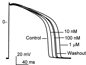
Fig. 1. Effect of morphine on action potentials. Action potentials were recorded from a representative rabbit ventricular myocyte, showing that action potential duration is prolonged and resting membrane potential is slightly hyperpolarized by the application of morphine at 0.01, 0.1, and 1 \mu\text{M} (6 min for each concentration). The effect was only partially reversed upon drug washout (10 min).
