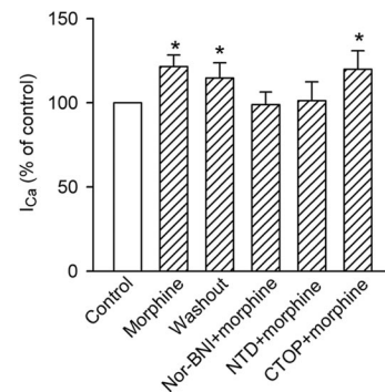
Fig. 4. Opioid receptor antagonists and morphine effects on L-type \text{Ca}^{2+} current ( I_{CaL} ). I_{CaL} was increased by the administration of 0.1 \mu\text{M} morphine, and the increase was partially reversed upon drug washout for 10 min. Pretreatment (5 min) with nor-binaltorphimine (nor-BNI, 5 \mu\text{M} , n = 7 ) and naltrindole (NTD, 5 \mu\text{M} , n = 8 ), but not CTOP ( 5 \mu\text{M} , n = 6 ), prevented morphine-induced increase of I_{CaL} . Data are expressed as mean \pm SD. * P < 0.05 versus control.
